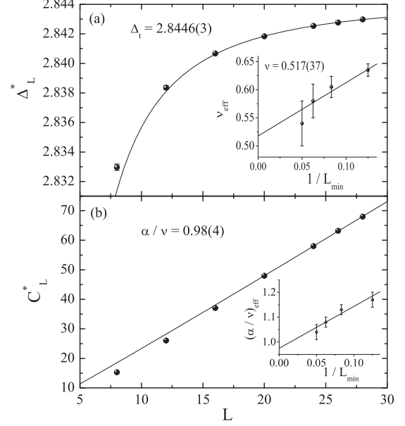
FIG. 9. Critical aspects of the 3D BC model at the tricritical point proposed in Ref. [14]: T_t = 1.4182 . (a) Shift behavior of \Delta_L^* obtained from the location of the specific-heat peaks. The solid line is a power-law fit of the form (8) for L \geq L_{\min} = 20 . The inset illustrates the infinite-volume extrapolation of the correlation-length effective exponent by varying the lower cutoff L_{\min} of the fits. (b) Scaling behavior of the specific-heat peaks again for the larger system sizes. The corresponding inset shows an infinite-volume extrapolation of the effective exponent ratio \alpha/\nu using the same procedure as in (a).
