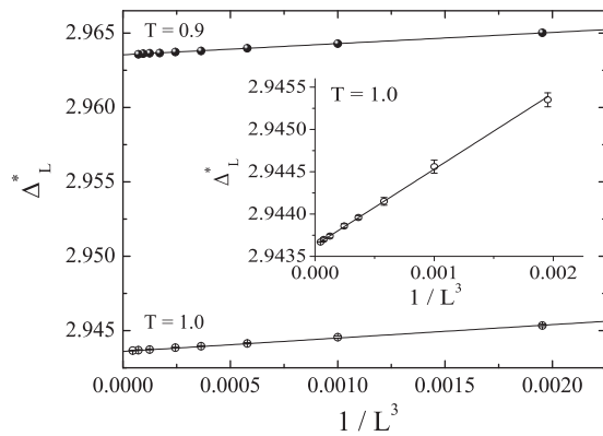
FIG. 6. Shift behavior (9) of the pseudocritical fields \Delta_L^* obtained from the peak location of the specific-heat curves (a sample of which is shown in Fig. 5) for both temperatures T = 1.0 and T = 0.9 in the first-order regime of the phase diagram. The obtained transition fields \Delta^* are given in the main text. The inset is a mere enlargement of the \sim L^{-d} approach of the pseudotransition points \Delta_L^* to L \rightarrow \infty for the temperature T = 1.0 .
