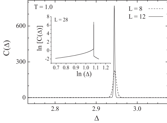
FIG. 5. Specific-heat curves as a function of the crystal field \Delta at T = 1.0 and two system sizes L = 8 (dashed line) and L = 12 (solid line). The inset illustrates a typical first-order-like specific-heat curve for a system with linear size L = 28 on a double logarithmic scale.
