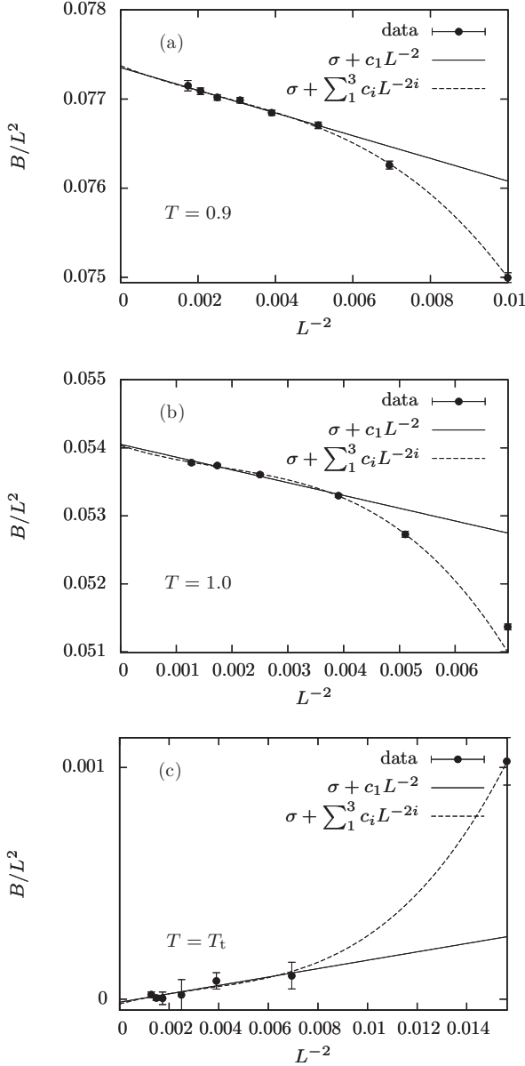
FIG. 8. Scaling of the barrier height B for all considered temperatures T \leq T_t . This barrier may be associated with the transition from a spin-0 dominated to a spin- \pm 1 dominated regime (see Fig. 2). Then B/L^2 plays the role of an interface tension for spin-0 strips.
