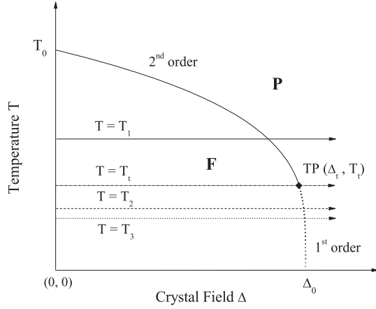
FIG. 1. General sketch of the phase diagram of the 3D BC model in the temperature–crystal-field plane. The phase boundary separates the ferromagnetic ( F ) phase from the paramagnetic ( P ) phase, in which the solid line indicates continuous phase transitions and the dotted line first-order phase transitions. The two lines merge at the tricritical point (TP), as highlighted by the black diamond. The limiting cases of T = 0 and \Delta = 0 are marked on the relevant axis with \Delta_0 = 3 and T_0 = 3.195(1) [22], respectively. The horizontal arrows illustrate the direction of crossing the phase boundary at fixed temperatures, studied in this work, in both the second-order ( T_1 = 2.0 ) and the first-order ( T_2 = 1.0 and T_3 = 0.9 ) regimes, as well as in the vicinity of the tricritical point ( T_t = 1.4182 ) [14].
