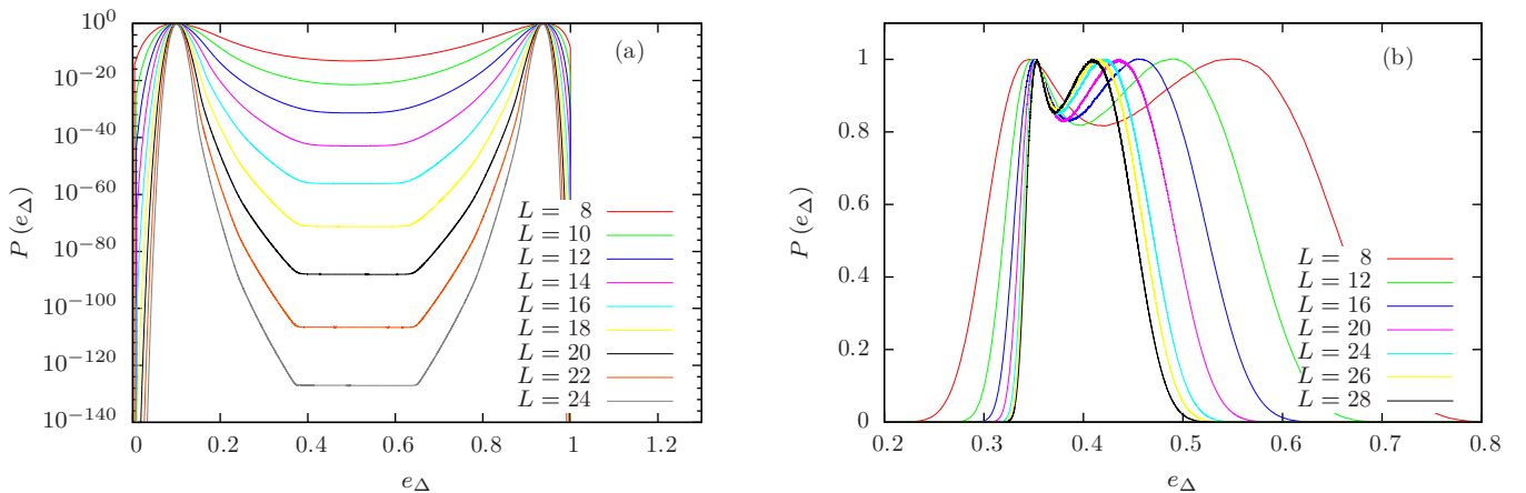
FIG. 2. (Color online) Illustration of the reweighted probability distribution at the transition field \Delta_{\text{eqh}} with respect to e_\Delta = E_\Delta/V at (a) T = 0.9 , which is well inside the first-order regime of the system (note the strongly increasing barrier with the system size), exhibiting a major suppression of intermediate states which is common for first-order transitions, and at (b) T = T_t = 1.4182 , which is in the vicinity of the tricritical point.
