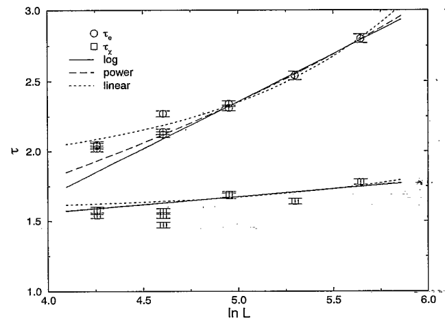
FIG. 1. The autocorrelation times of energy, \tau_e , and susceptibility, \tau_\chi at the simulation point K_0=0.263 , together with various types of fits to the data of the three largest lattices as discussed in the text.
