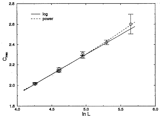
FIG. 8. Finite-size scaling of the specific-heat maxima C_{\max} . Also shown are least-squares fits to a logarithmic ansatz, C_{\max}=B_0+B_1\ln L [with B_0=0.346(52) , B_1=0.391(12) ], and to a pure power-law ansatz, C_{\max}=cL^{\alpha/\nu} [with c=0.926(22) , \alpha/\nu=0.1824(53) ].
