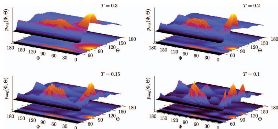
FIG. 1. (Color) Bond and torsion-angle distributions of sequence S3 at different temperatures. The distributions of the torsion angles are reflection symmetric and therefore only the positive intervals are shown.
