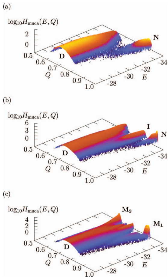
FIG. 4. (Color) Multicanonical histograms H_{\text{muca}}(E, Q) of energy E and angular overlap parameter Q for the three sequences (a) S1, (b) S2, and (c) S3. The different branches of these distributions are channels which the heteropolymer can follow in the folding process towards the native state. The native folds are located in the right corner for Q=1 and E=E_{\text{min}} . Folding channels are labeled as D (denatured states), N (native folds), I (intermediates), and M (metastable states).
