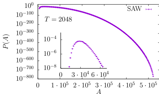
Whole distribution of the area A of the convex hull of SAWs.
