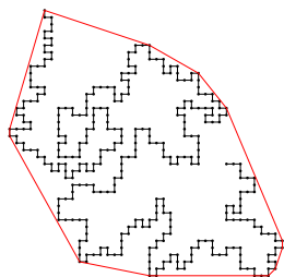
Convex Hull of a Self-Avoiding Random Walk (SAW)
