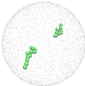
Bead-Spring Polymers
