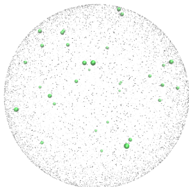
Lennard-Jones Gas
