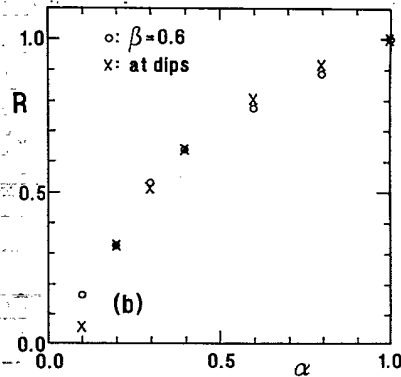
FIG. 5. (a) Ratio R = M_3/M_1 of vortex-loop elements. (b) The same data as in (a) replotted vs \alpha for fixed \beta=0.6 ( \circ ) and at the dips ( \times ).
