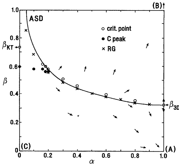
FIG. 1. Phase diagram in the \alpha - \beta plane. The continuous line shows the critical points estimated by the approximate self-duality (ASD). The symbols ( \circ ) and ( \bullet ) are the critical points and specific-heat maxima determined from Monte Carlo (MC) simulations with L=16 . The symbols ( \times ) are the critical points given by the Migdal renormalization group (RG). The arrows illustrate typical flows of RG into the infrared region.
