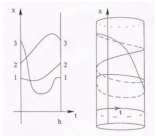
FIG. 1: The worldlines of three particles that, after moving a time \tau = \hbar/k_B T in the imaginary time direction, are cyclically permuted (left panel). The three separate worldlines can also be represented by a single worldline that winds three times around the imaginary time axis (right panel). (After Ref. [4].)
