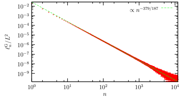
FIG. 5: Distribution \ell_n^G normalized to the volume L^2 of geometrical clusters in the 2D Ising model at criticality on a square lattice of linear size L = 512 . Statistical error bars are omitted from the data points for clarity. The straight line is a one-parameter fit through the data points with (minus) the slope fixed to the value \tau^G = 379/187 = 2.02673\dots . The fit illustrates that asymptotically the distribution is algebraic at criticality.
